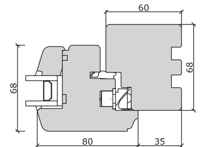
Cill Extension (Various sizes available)
