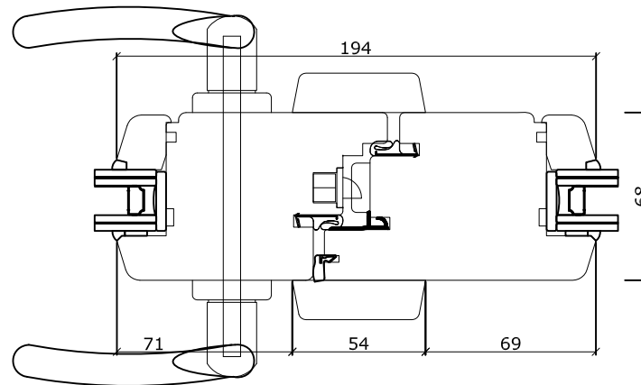
Contemporary Range Inward Opening Flying Mullion - Single Handle
