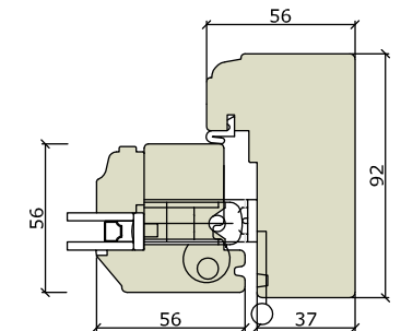
Cill Extension (Various sizes available)
