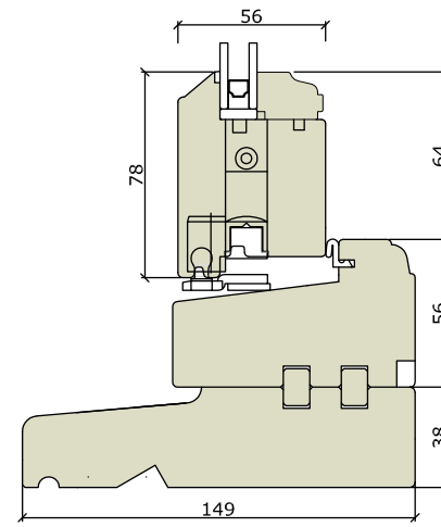
Sub-Cill (Various sizes available)
