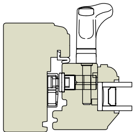
Sub-Cill (Various sizes available)
