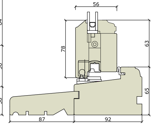
Cill Extension (Various sizes available)
