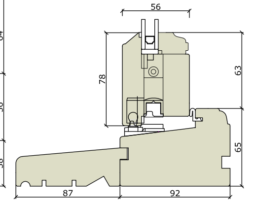
Cill Extension (Various sizes available)
