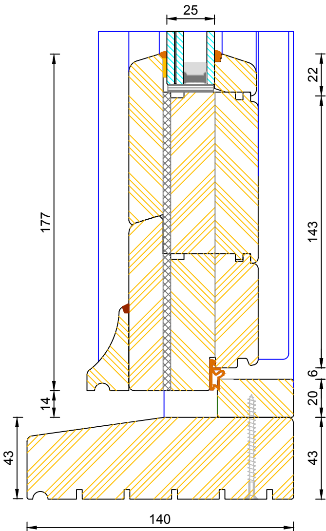
Section A1-A1
