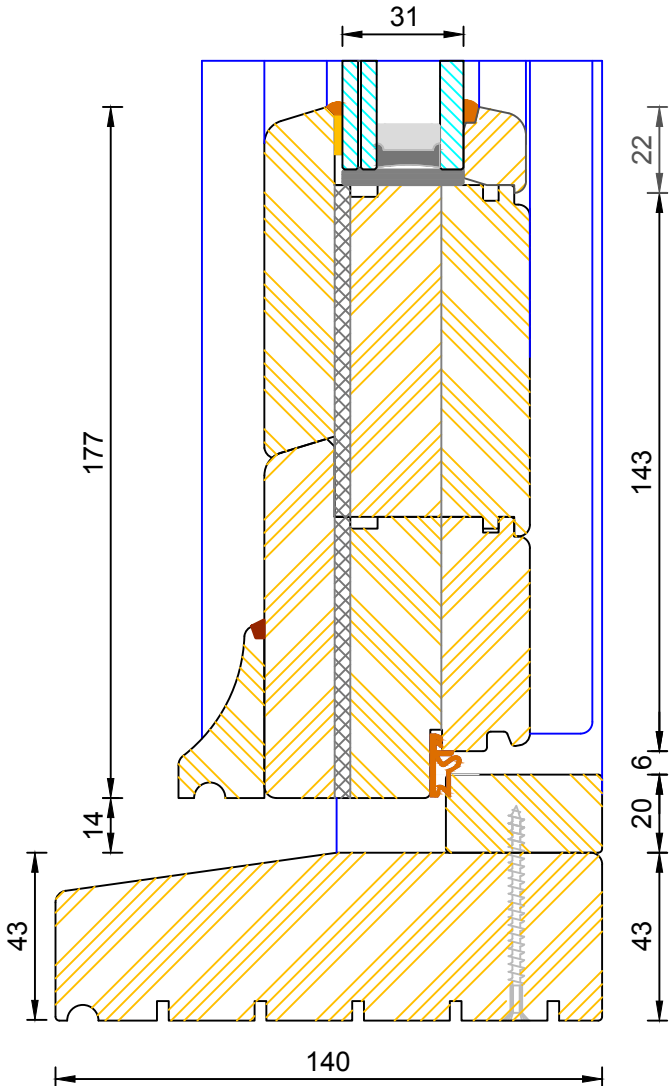
Section A1-A1
