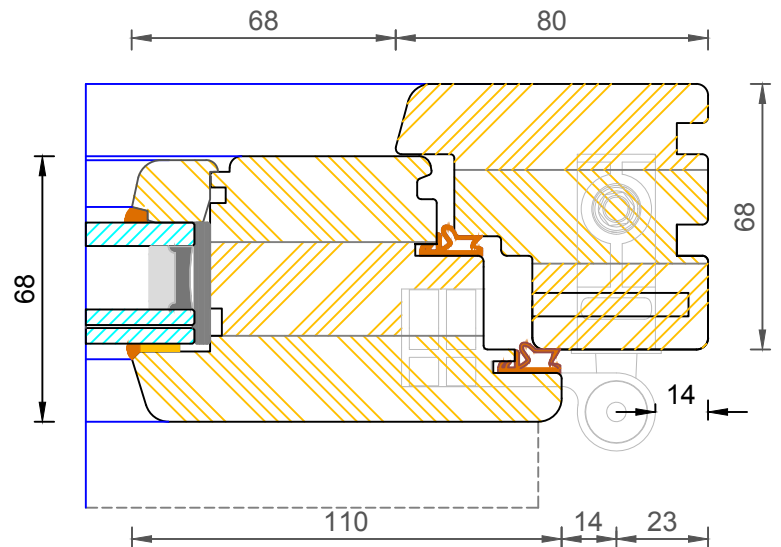
Section B1-B1
